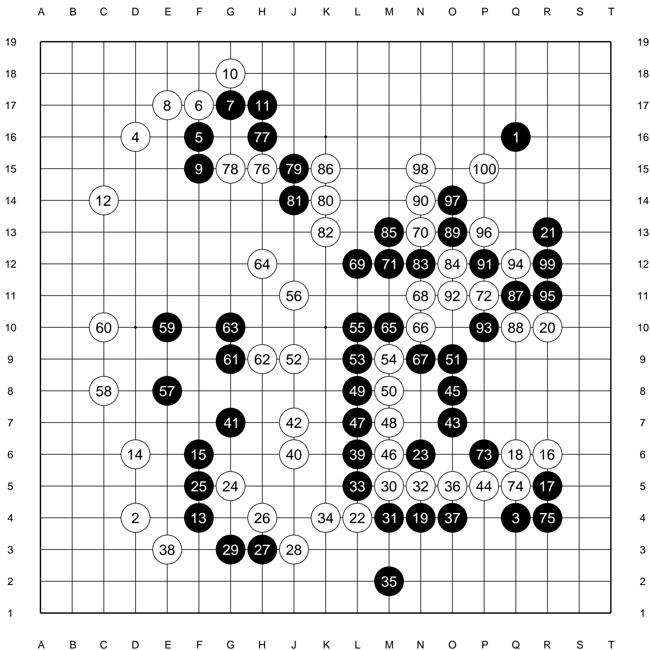
Game 1 - Figure 1 (1-100)
